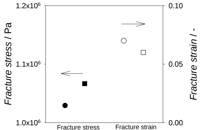
Fig.5 Fracture stress (black) and fracture strain (white) for sample A (circle) and B (square). Measurements were made at 20 °C.
